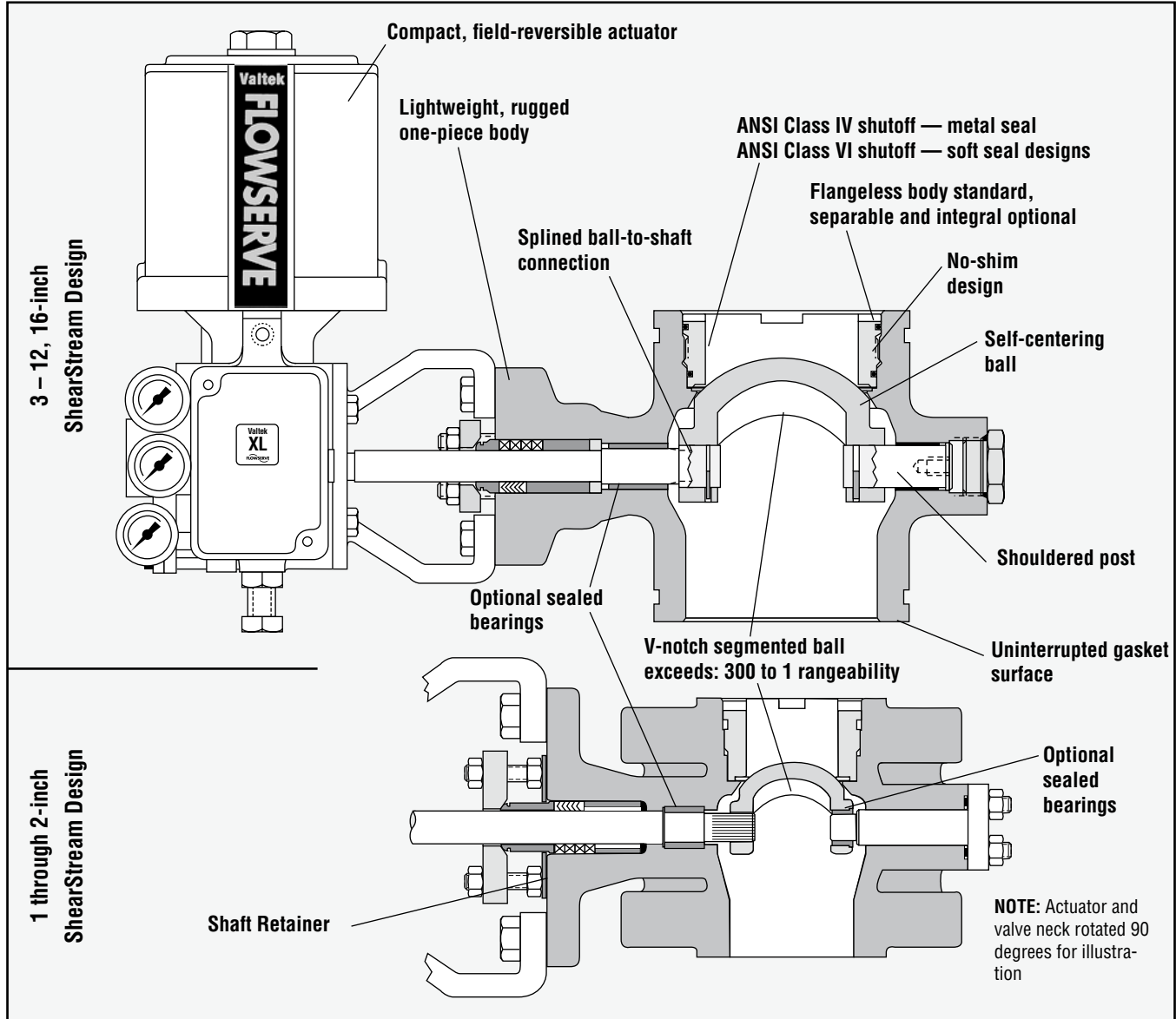
Figure 1: ShearStream Design
