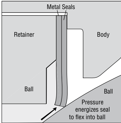
Figure 2: Metal seat: shaft downstream
